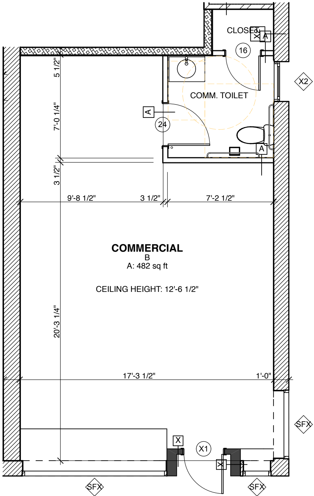
FIRST FLOOR UNIT PLAN SCALE: 1/4" = 1'-0"
